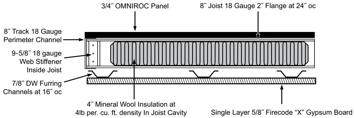
END VIEW
